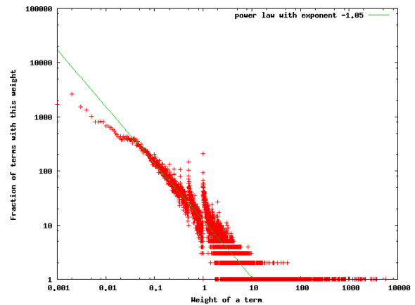
Figure 1: Distribution of weights of terms in |A| .
