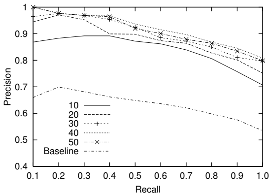
Figure 5: Varying the number of results per query
